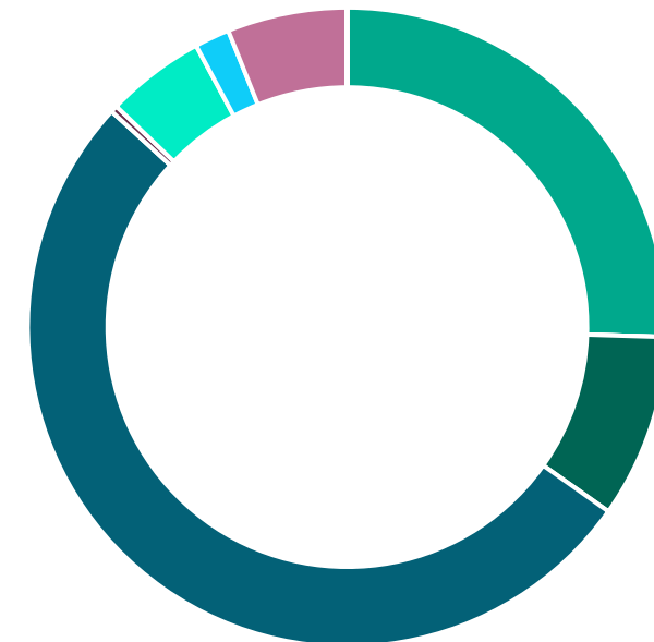
Contribution Methods
